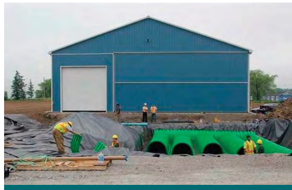
Figure 2.7.2: In this design, rainwater is collected in a modular subsurface system and used for emergency fire suppression. (Source: Aquafor Beech)
