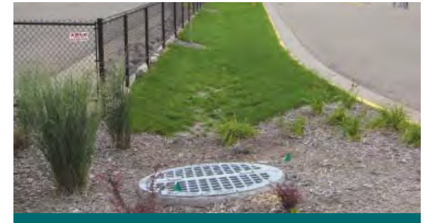
Figure 2.4.1: A long island separating an entranceway and parking lot is used to treat runoff with a bioswale. (Source: CVC)
