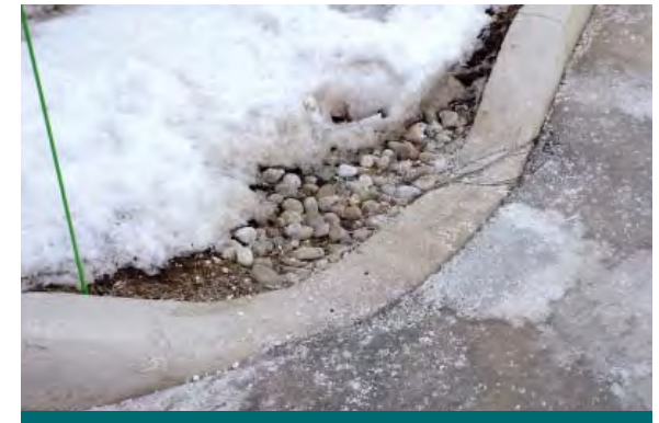
Figure 4.9.3: This curb cut had to be cleared to allow water to flow into the practice. (Source: CVC)
