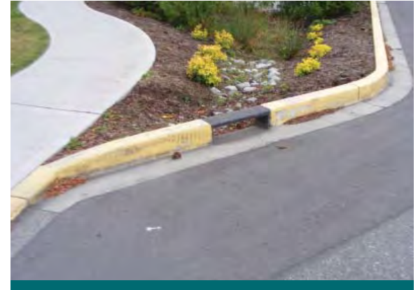
Figure 6.4.10: A cover on a curb cut can provide a barrier that prevents damage from snow removal operations. (Source: Aquafor Beech)
