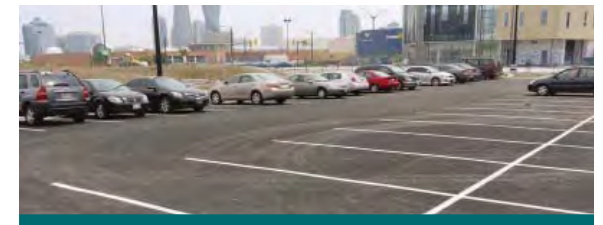
Figure 2.2.2: Porous asphalt can look quite similar to conventional asphalt. Site operators should track the location of permeable infrastructure to ensure that it is not paved over by future paving projects. (Source: CVC)
