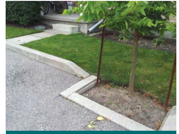
Figure 4.8.3: This parking area could be retrofitted with permeable pavement. The green area on the opposite side of the curb provides a suitable location for a small bioretention planter accepting roof runoff. (Source: Aquafor Beech)
