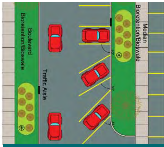
Figure 6.4.16: 90°, 60°, and 45° parking stall configurations. (Source: Aquafor Beech)
