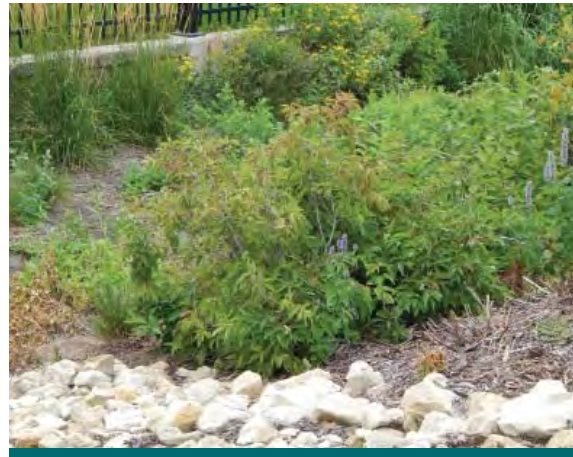
Figure 6.4.26: Well-vegetated bioswales at the University of Minnesota. (Source: Aquafor Beech)
