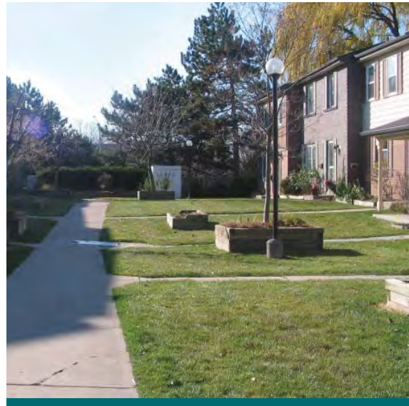
Figure 4.8.2: In many low-rise residential developments, a portion of the roof drainage is directed to conveyance features (ie. rear-yard catchbasins). In the Ganonoque townhouse complex in Mississauga, homes and common elements are built on top of the parking garage, extending the life of the parking lots. (Source: CVC)
