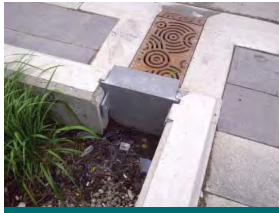
Figure 6.4.9: A gate has been added to this grated curb cut design to allow the facility to be closed during the winter. (Source: Aquafor Beech)
